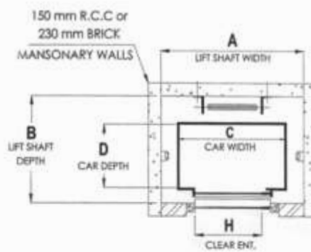
LIFT SHAFT PLAN
