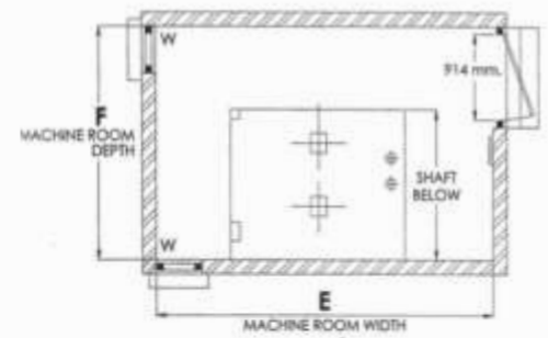
MACHINE ROOM PLAN
